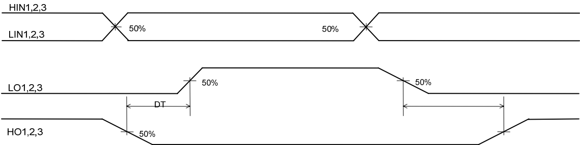
Fig. 4. Internal Deadtime Timing Waveforms
